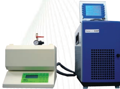
K-Factor Machine Measuring the thermal insulation properties of polyurethane foam systems.
